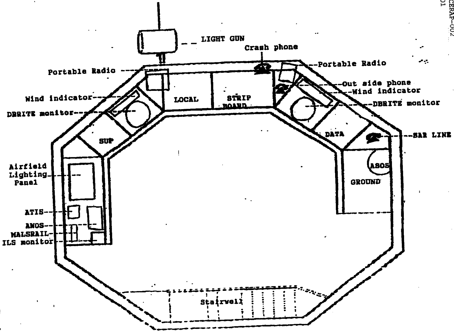
TOWER CAB LAYOUT
