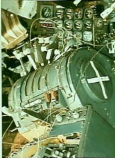
Photo 17: Throttle Quadrant
